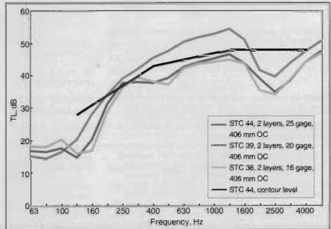
Figure 5. Transmission loss per frequency for a 1+1 layer partition with studs installed at 406 mm OC for various stud gages.
