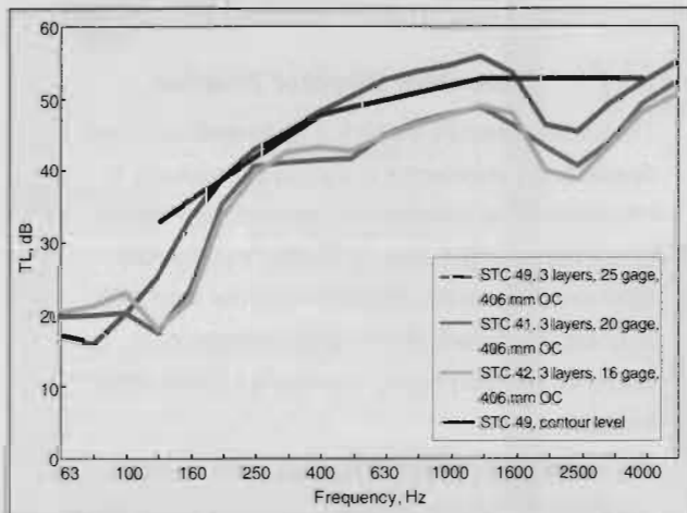
Figure 3. Transmission loss per frequency for a 2+1 layer partition with studs installed at 406 mm OC for various stud gages.
