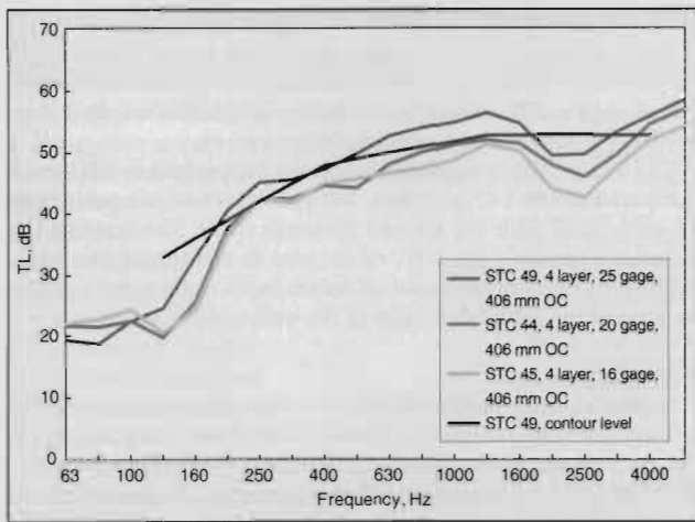
Figure 1. Transmission loss per frequency for a 2+2 layer partition with studs installed at 406 mm OC for various stud gages.
