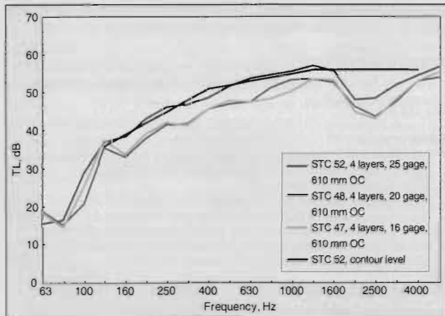
Figure 2. Transmission loss per frequency for a 2+2 layer partition with studs installed at 610 mm OC for various stud gages.
