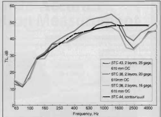
Figure 6. Transmission loss per frequency for a 1+1 layer partition with studs installed at 610 mm OC for various stud gages.
