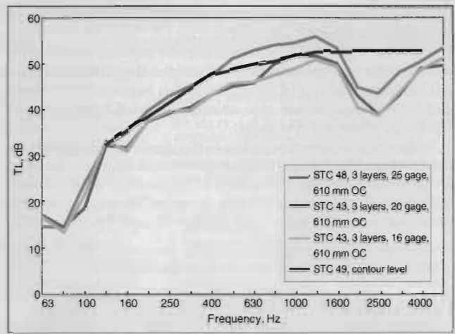
Figure 4. Transmission loss per frequency for a 2+1 layer partition with studs installed at 610 mm OC for various stud gages.
